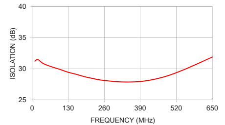
LRPS-2-1W-75+ ISOLATION
