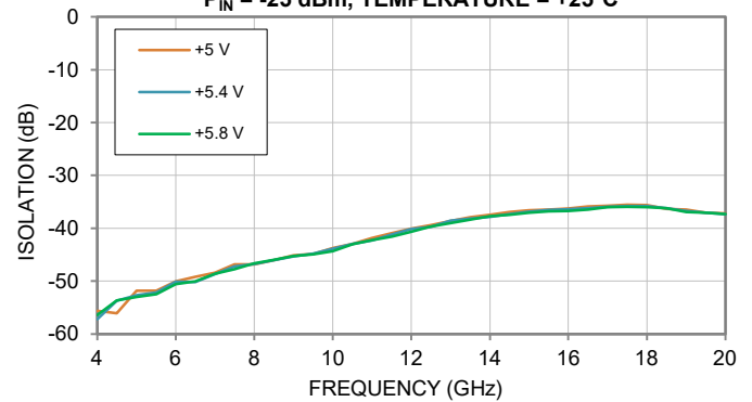
ISOLATION vs. BASE VOLTAGE ( V_B ) P_{IN} = -25 dBm, TEMPERATURE = +25°C
