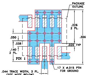
Demo Board MCL P/N: TB-956+ Suggested PCB Layout (PL-045)
