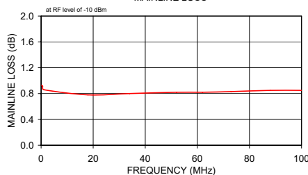
PDC-10-6-75 MAINLINE LOSS
