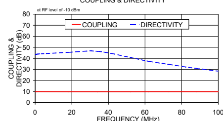
PDC-10-6-75 COUPLING & DIRECTIVITY
