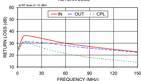
PDC-20-3-75 RETURN LOSS
