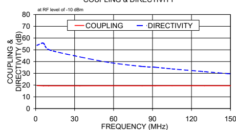
PDC-20-3-75 COUPLING & DIRECTIVITY
