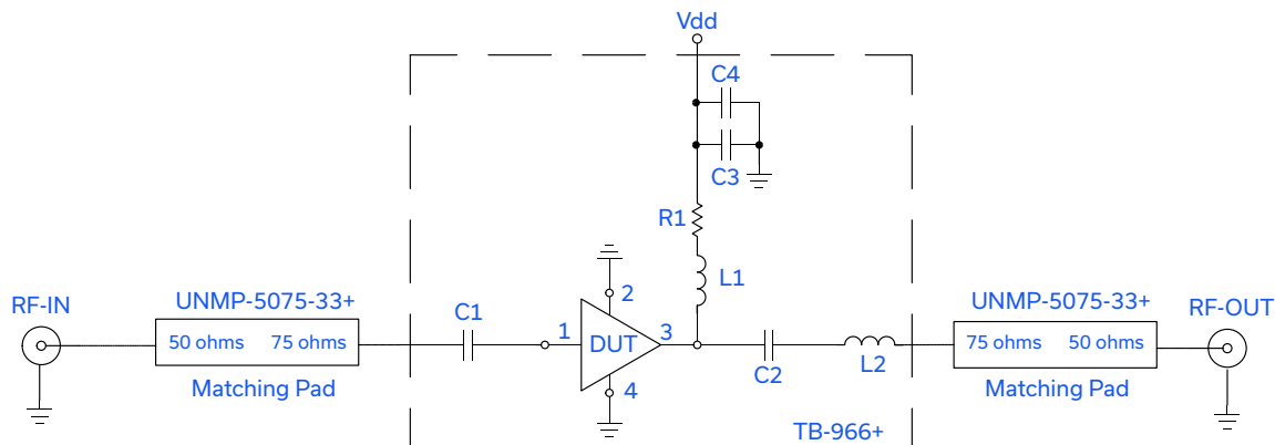
Fig 1A. Block Diagram of Test Circuit used for characterization. (DUT soldered on TB-966+) Gain, Return loss, Output power at 1dB compression (P1 dB) , output IP3 (OIP3), output IP2 (OIP2) and noise figure measured using Agilent's N5242A PNA-X microwave network analyzer & E5071C ENA Series Network Analyzer.
