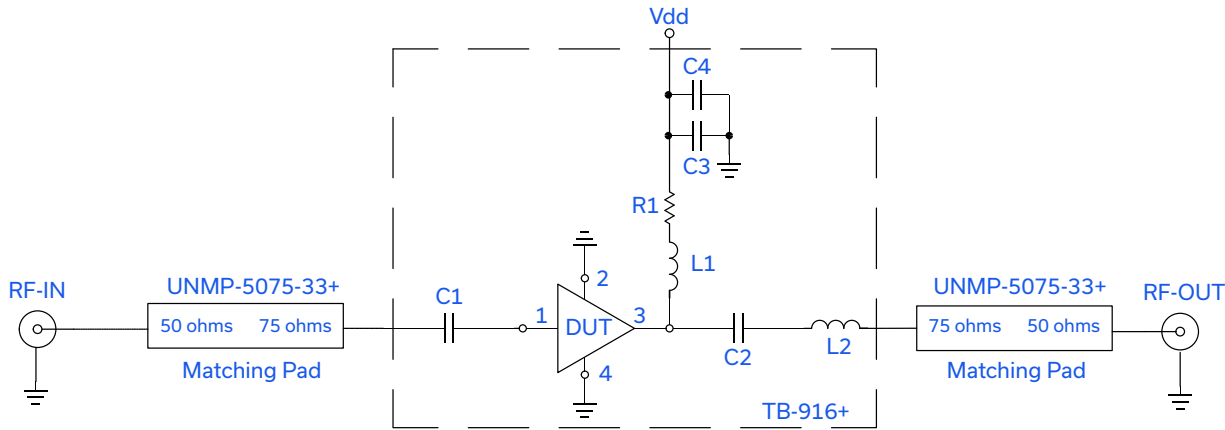
Fig 1B. Block Diagram of Test Circuit used for characterization. (DUT soldered on TB-916+) Gain, Return loss, Output power at 1dB compression (P1 dB) , output IP3 (OIP3), output IP2 (OIP2) and noise figure measured using Agilent's N5242A PNA-X microwave network analyzer & E5071C ENA Series Network Analyzer.
