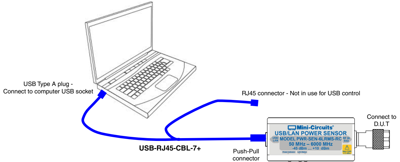
Connection diagram for USB control
