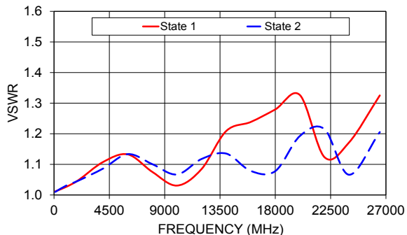
VSWR (J1)
