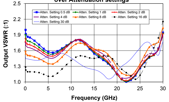
Output VSWR over Attenuation settings
