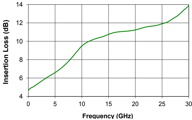
Insertion Loss
