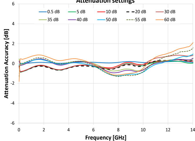
Attenuation Accuracy @ 50°C vs. Frequency over Attenuation settings
