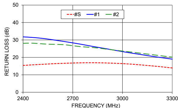
RETURN LOSS
