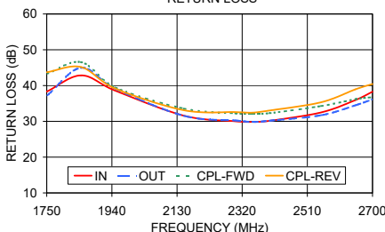
SYBD-16-272HP+ RETURN LOSS
