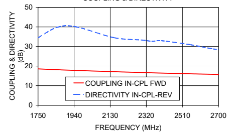
SYBD-16-272HP+ COUPLING & DIRECTIVITY
