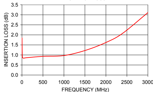
TC1-33-75G2+ INSERTION LOSS
