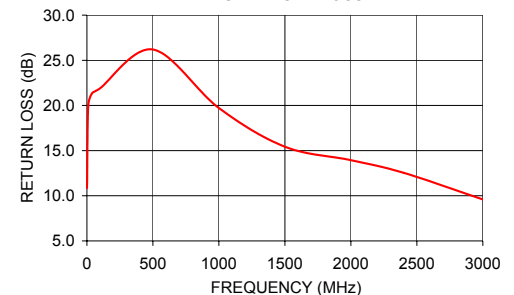
TC1-33-75G2+ INPUT RETURN LOSS
