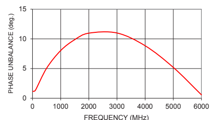
TCM1-63AX-2+ PHASE UNBALANCE
