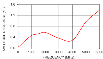
TCM1-63AX-2+ AMPLITUDE UNBALANCE
