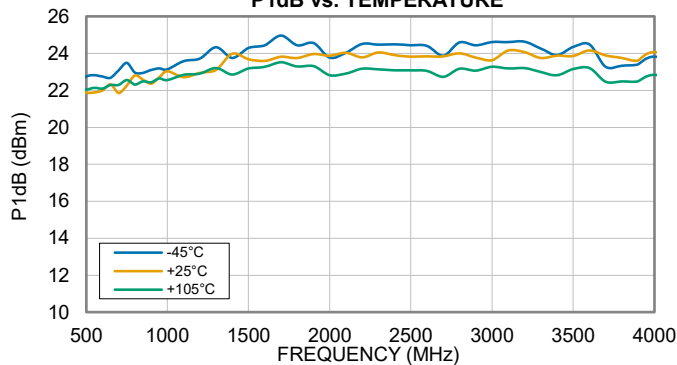
P1dB vs. TEMPERATURE
