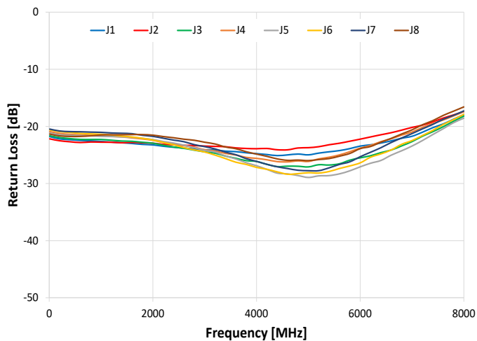
Return Loss, COM over Temperature (J1 Active)
