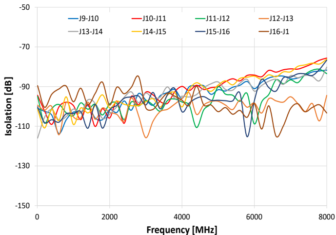
Isolation, Ports J9 - J16 Terminated
