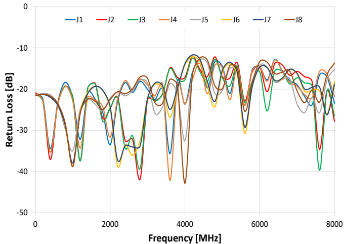
Return Loss, Ports J1 - J8 Terminated
