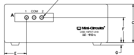
FRONT VIEW (SCALE 1.5:1)
