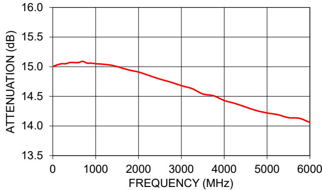
VAT-15W2+ ATTENUATION
