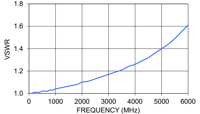
VAT-15W2+ VSWR
