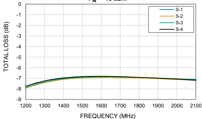
TOTAL LOSS 3 @ TEMPERATURE = +25°C P IN = -10 dBm
