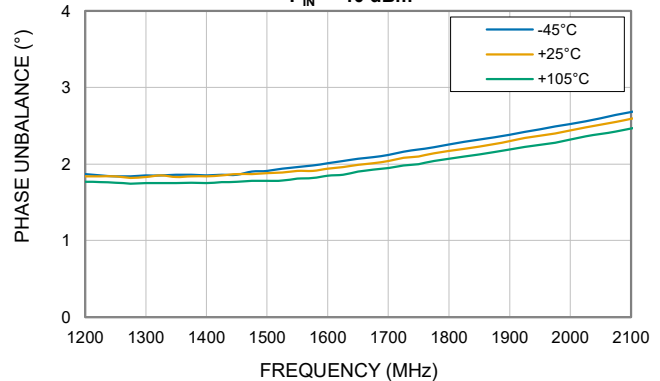
PHASE UNBALANCE vs TEMPERATURE, P IN = -10 dBm
