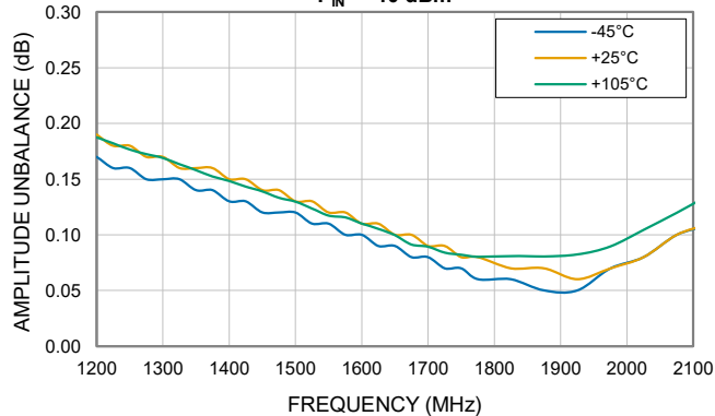
AMPLITUDE UNBALANCE vs TEMPERATURE, P IN = -10 dBm
