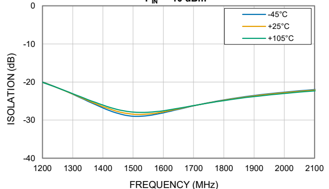
ISOLATION 2-3 vs TEMPERATURE, P IN = -10 dBm
