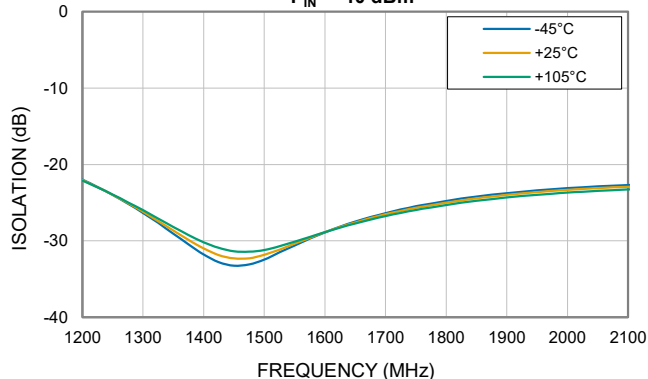
ISOLATION 1-2 vs TEMPERATURE, P IN = -10 dBm
