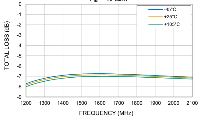
TOTAL LOSS 4 vs TEMPERATURE, P IN = -10 dBm
