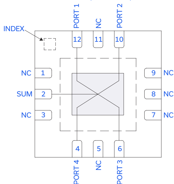
Figure 1. WP4G1A+ Functional Diagram
