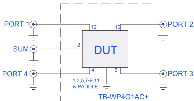
Figure 2. WP4G1A+ Characterization and Application Circuit
