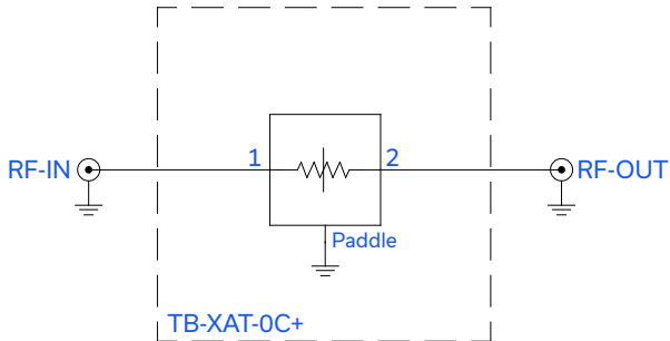
Figure 2. XAT-0+ Characterization and Application Circuit.
