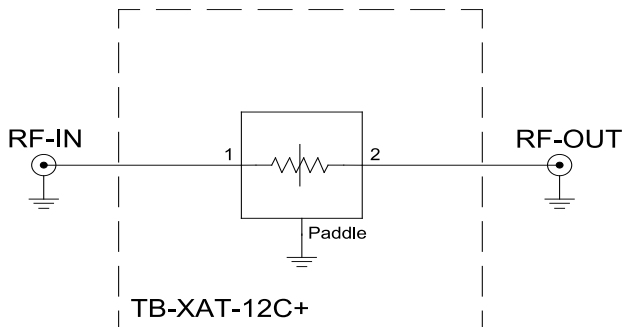
Figure 2. XAT-12+ Characterization and Application Circuit.
