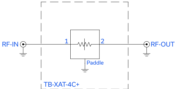
Figure 2. XAT-4+ Characterization and Application Circuit.
