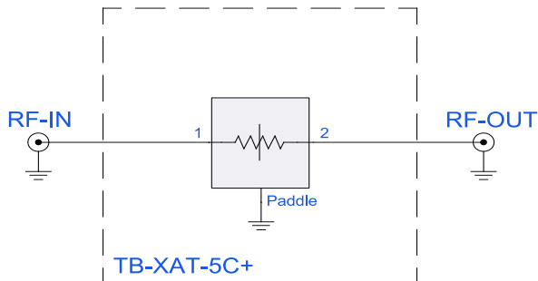
Figure 2. XAT-5+ Characterization and Application Circuit.
