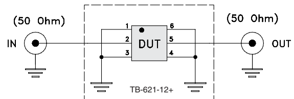
Fig 1. Block diagram of Test Circuit used for characterization, Test board TB-621-12+ Conditions: Attenuation, VSWR: Pin=-10 dBm
