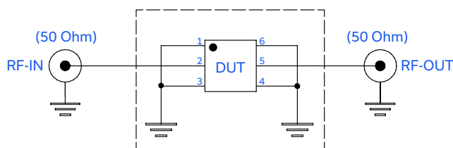
Fig 1. Block diagram of Test Circuit used for characterization, Test board TB-YAT-2A+ Conditions: Attenuation, VSWR: Pin=-10 dBm
