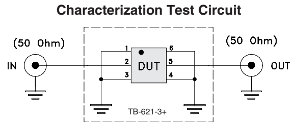
Fig 1. Block diagram of Test Circuit used for characterization, Test board TB-621-3+ Conditions: Attenuation, VSWR: Pin=-10 dBm
