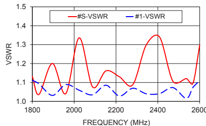
ZC16PD-2185-S+ VSWR
