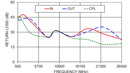
ZCDC20-5R263-S+ RETURN LOSS
