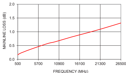
ZCDC20-5R263-S+ MAINLINE LOSS
