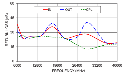
ZCDC30-K0644-S+ RETURN LOSS
