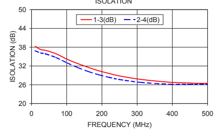
ZFSC-12-175 ISOLATION
