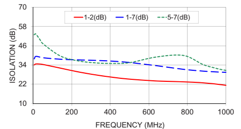
ZFSC-8-4-75+ ISOLATION
