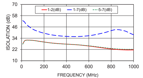
ZFSC-8-43-S+ ISOLATION
