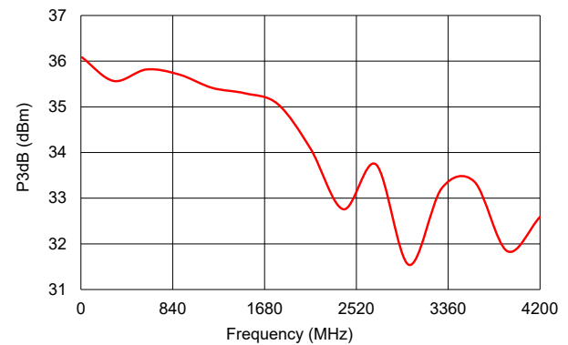
Output Power at 3dB Compression vs. Frequency
