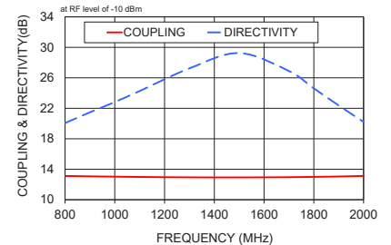
ZNDC-13-2G-S+ COUPLING & DIRECTIVITY
