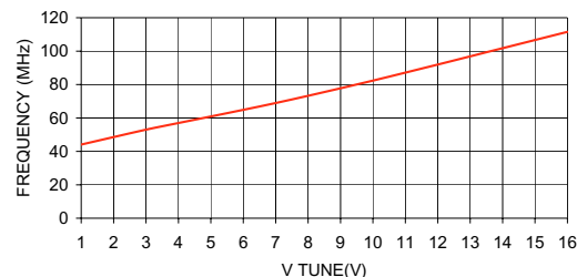
ZOS-100 FREQUENCY vs. TUNING VOLTAGE
