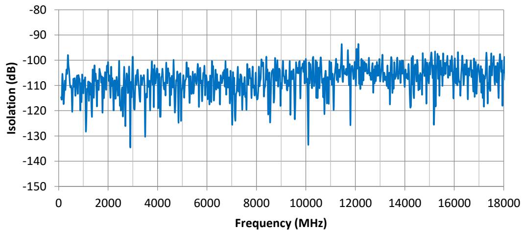
Isolation
