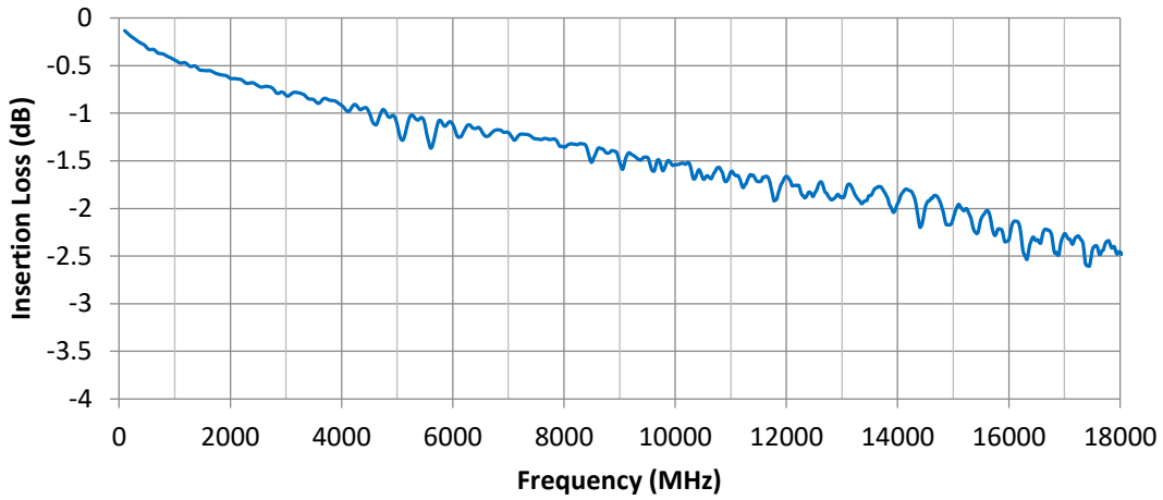
Insertion Loss
