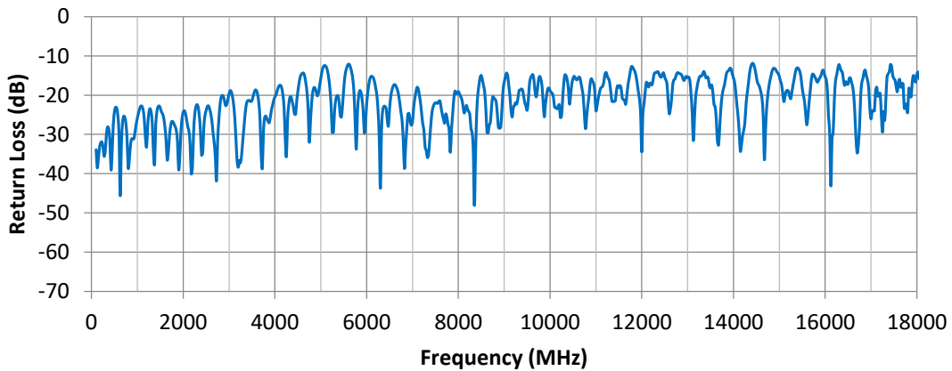
Return Loss
