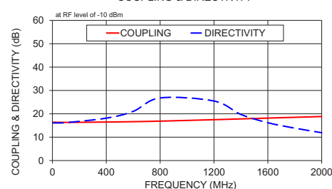
ZX30-17-5-S+ COUPLING & DIRECTIVITY
