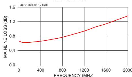
ZX30-17-5-S+ MAINLINE LOSS
