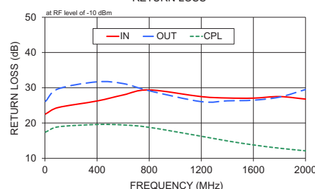
ZX30-17-5-S+ RETURN LOSS
