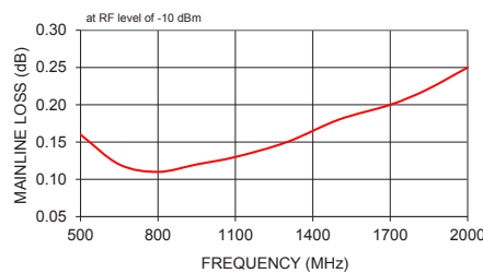
ZX30-20-20BD-S+ MAINLINE LOSS
