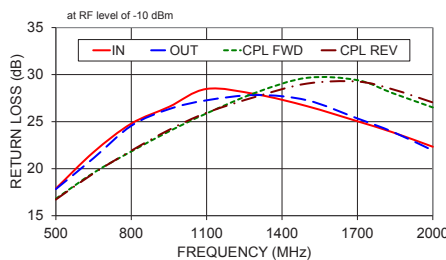
ZX30-20-20BD-S+ RETURN LOSS
