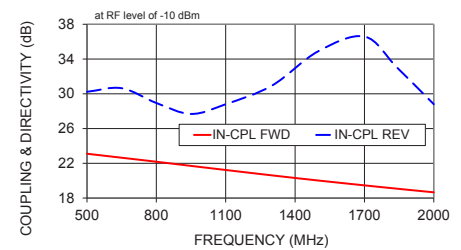
ZX30-20-20BD-S+ COUPLING & DIRECTIVITY
