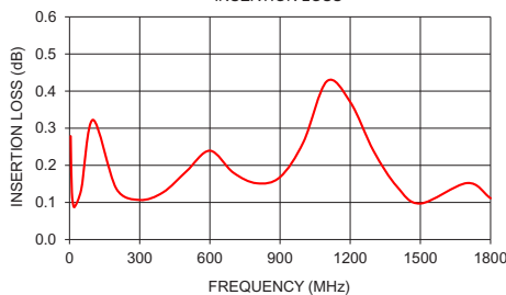
TACH-182-75+ INSERTION LOSS
