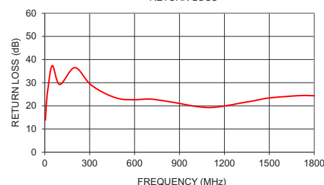
TACH-182-75+ RETURN LOSS
