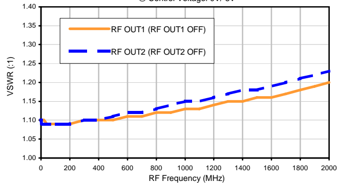
VSWR (OFF)
