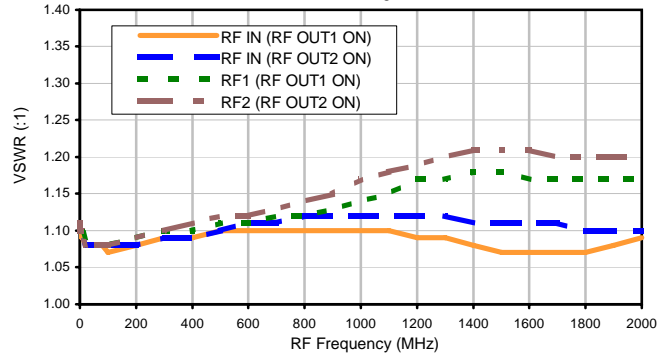
VSWR (ON)
