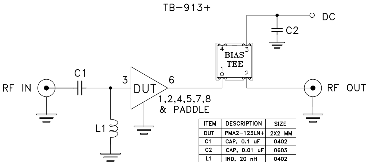
Schematic Diagram
