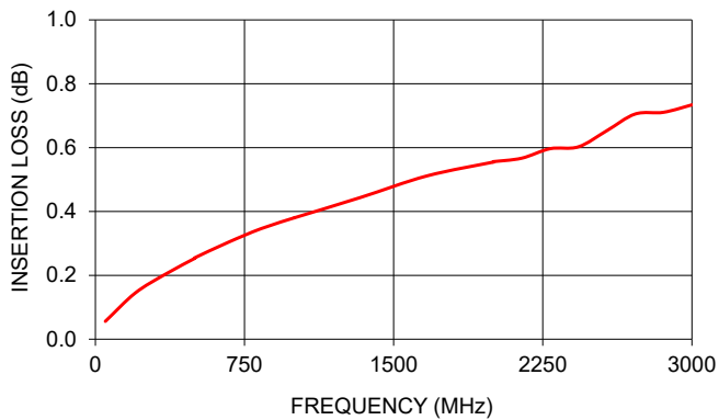
CBL-3FM-75+ INSERTION LOSS
