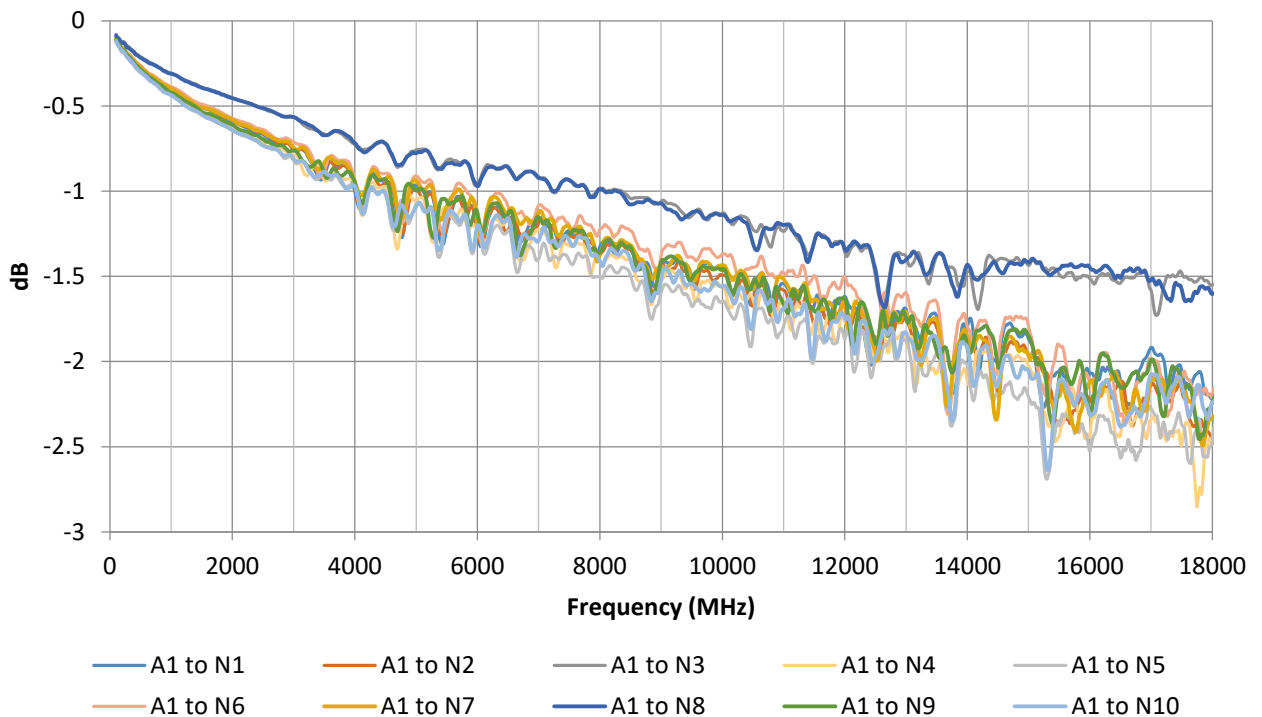
Insertion Loss
